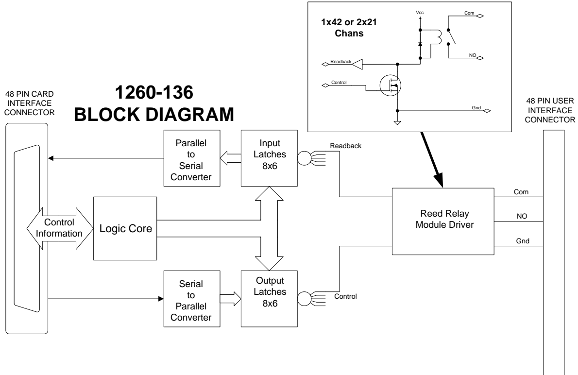
Figure 2-3, Block Diagram
